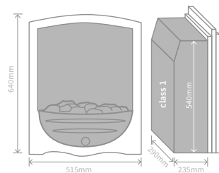
Freya Gas Open fronted Convactor Gas Fire
