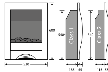
Zara* Radiant Gas Fire
