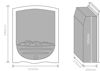
Freya Gas Glass fronted Convactor Gas Fire
