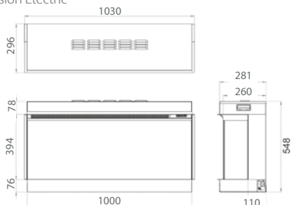
Chelsea 1000VS Illusion Electric
