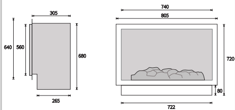
Chelsea Tall Built-in Gas Fire
