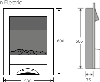
Zara Illusion Electric
