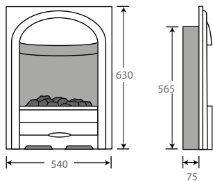
Carmen Inset Illusion Electric
