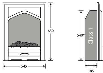
Churchill Radiant Gas Fire
