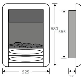
Chelsea 750VS Electric
